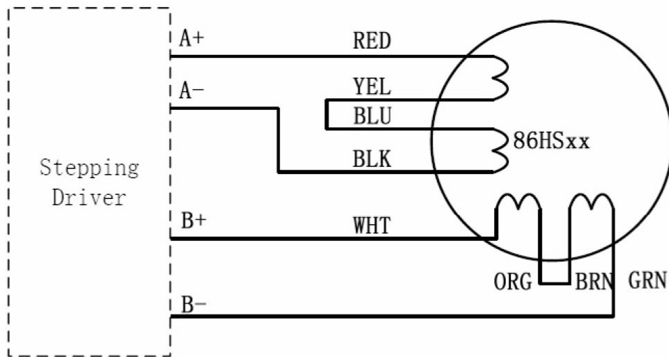
(a) 86HSxx series connection (8 leads)
