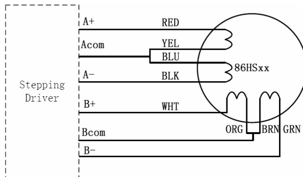
(c) 86HSxx unipolar connection (8 leads)
