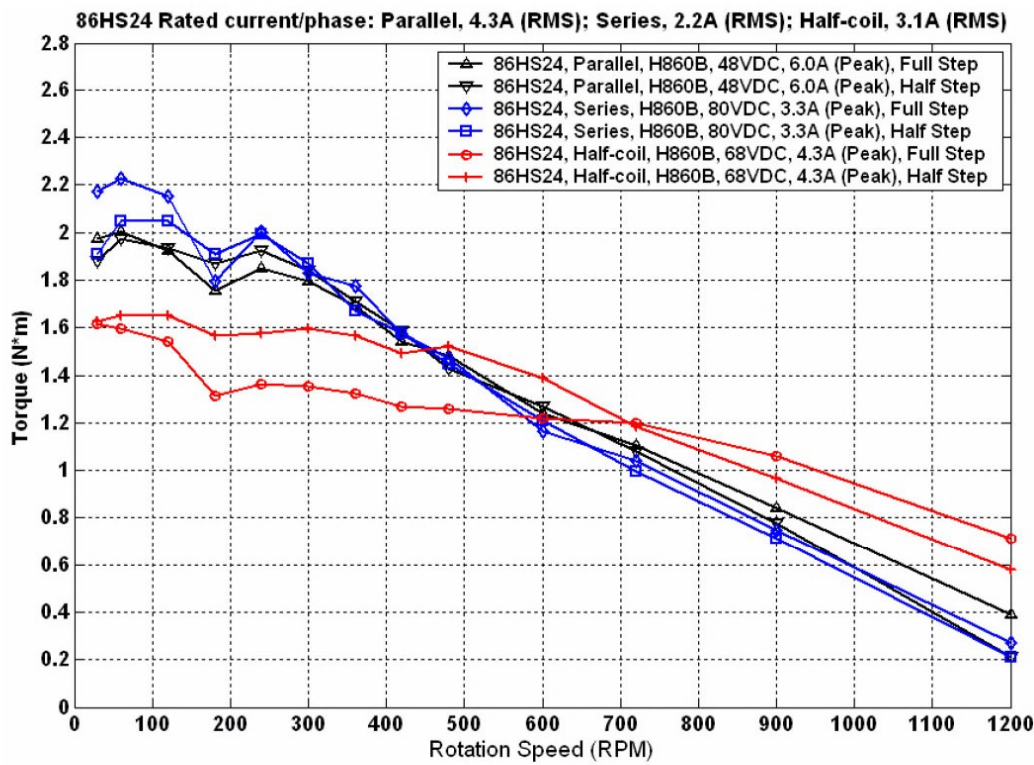
Figure 7: Speed-torque curves of the 86HS24
