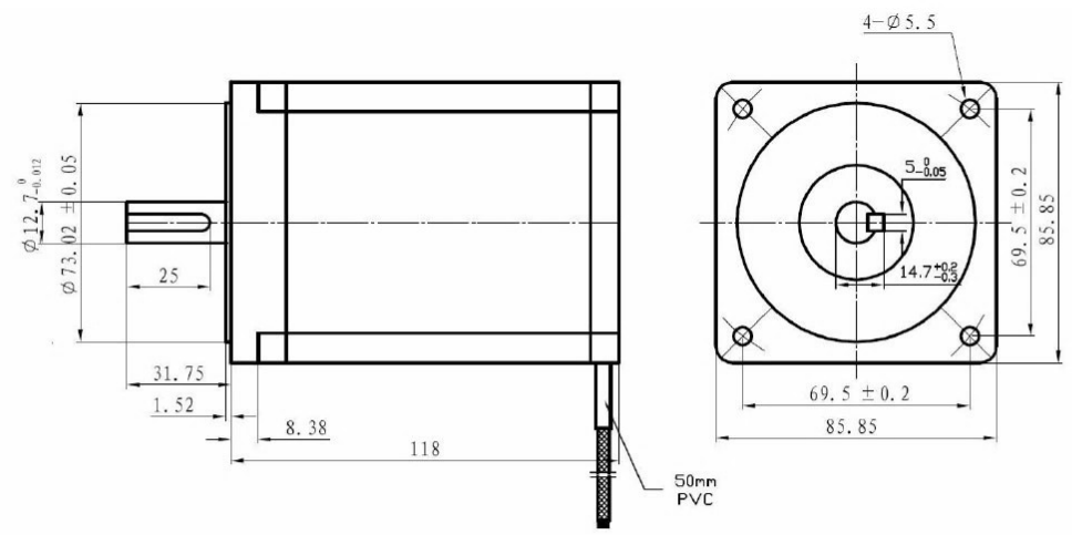
Figure 6: Mechanical specification of the 86HS85
