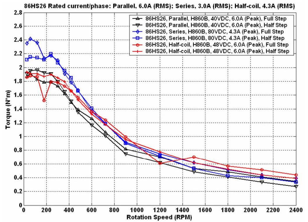
Figure 8: Speed-torque curves of the 86HS26
