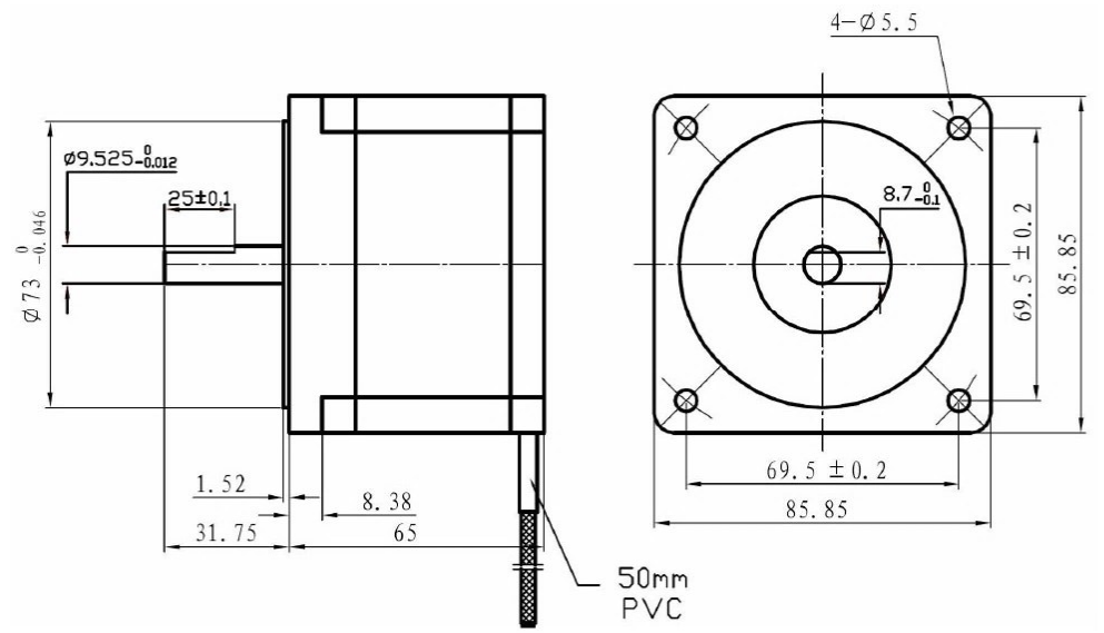
Figure 4: Mechanical specification of the 86HS35
