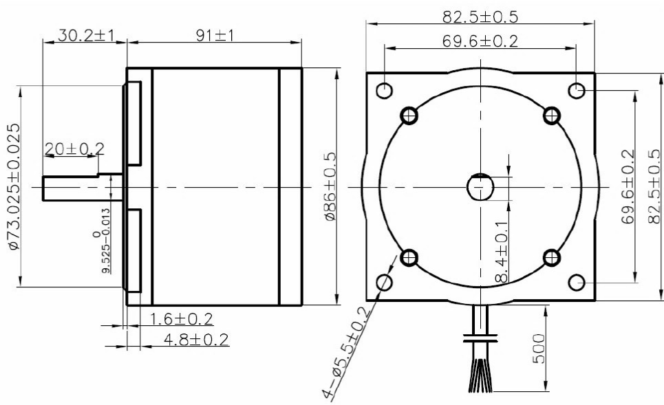
Figure 3: Mechanical specification of the 86HS38
