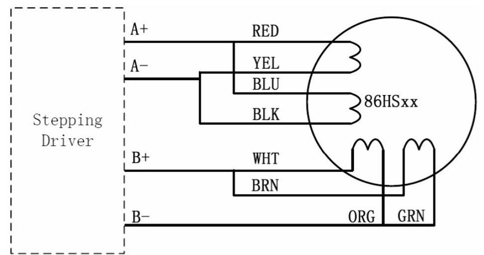
(b) 86HSxx parallel connection (8 leads)
