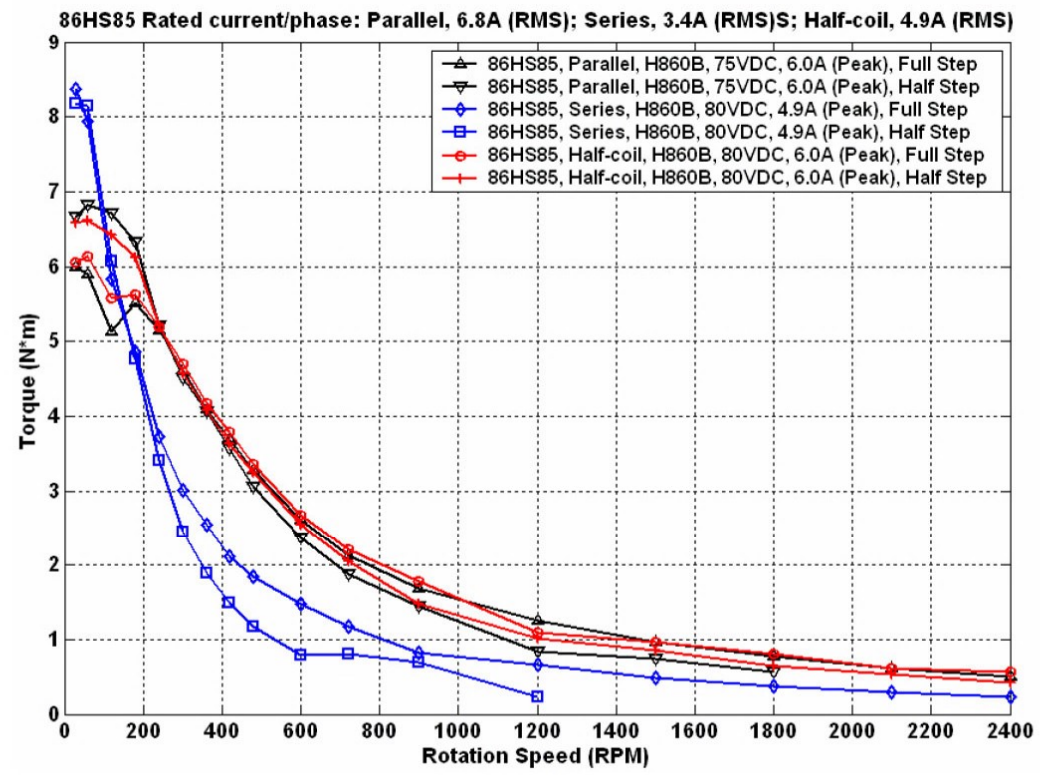
Figure 12: Speed-torque curves of the 86HS85
