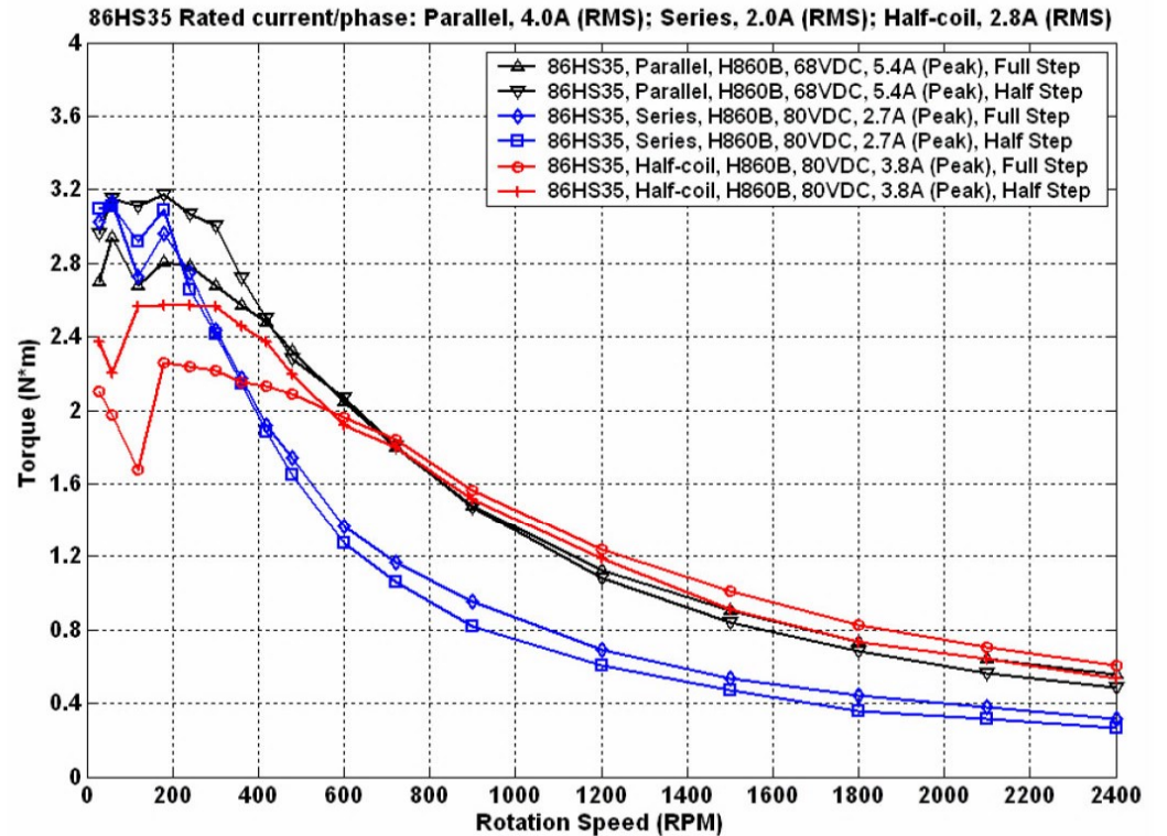
Figure 10: Speed-torque curves of the 86HS35
