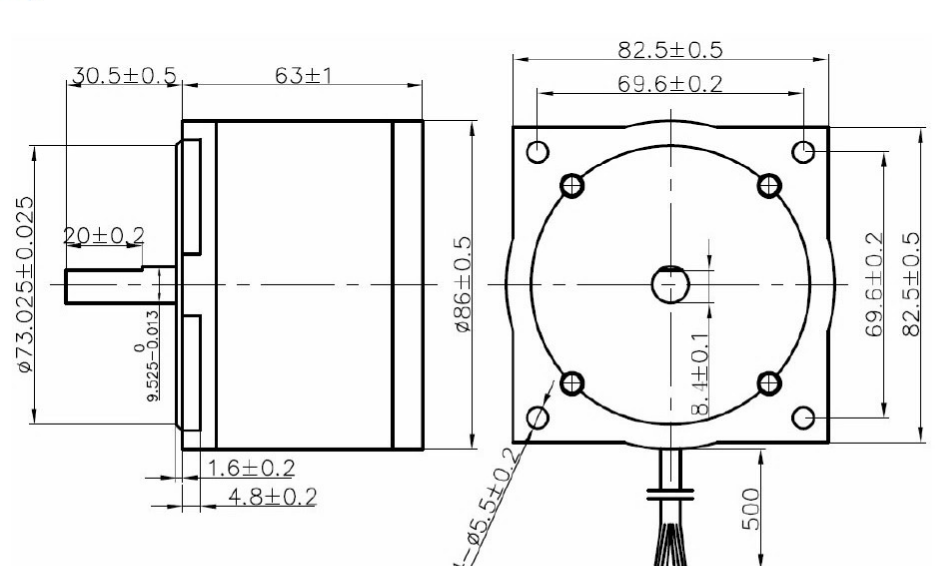
Figure 2: Mechanical specification of the 86HS26
