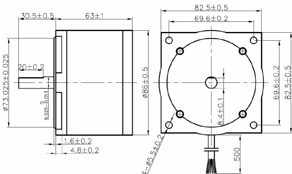
Figure 1: Mechanical specification of the 86HS24
