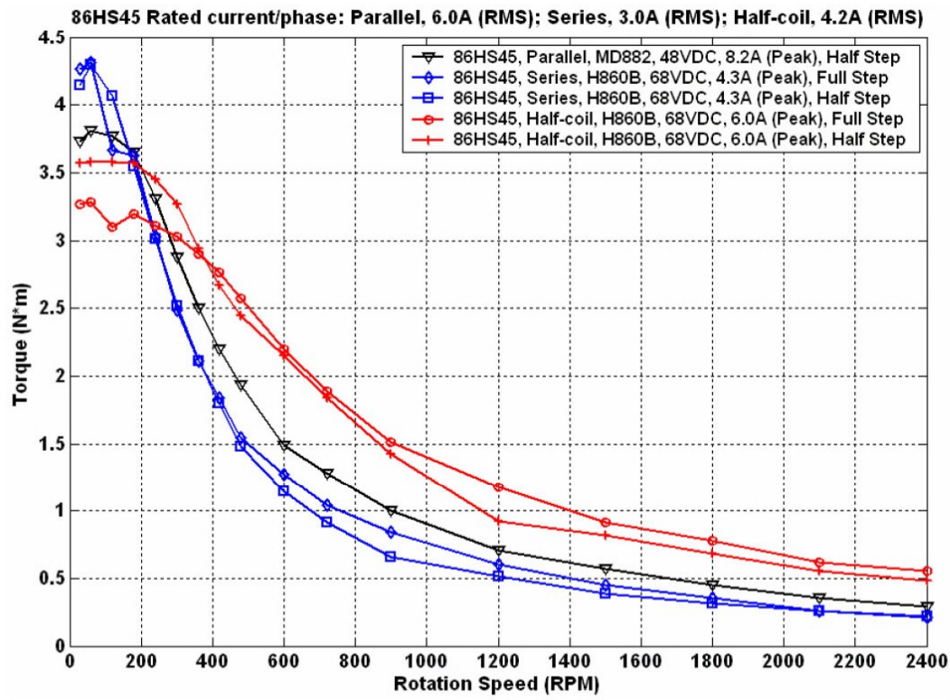
Figure 11: Speed-torque curves of the 86HS45
