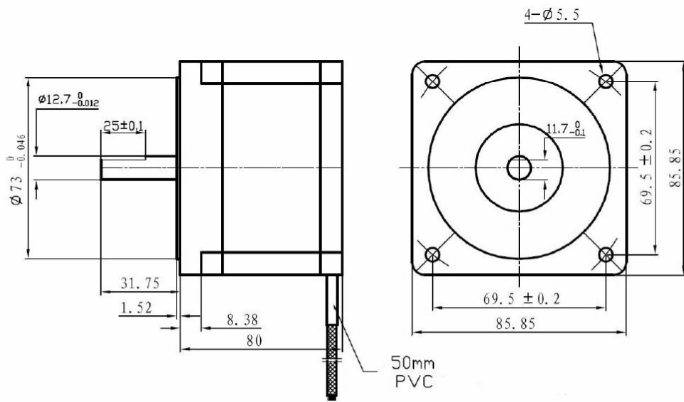
Figure 5: Mechanical specification of the 86HS45
