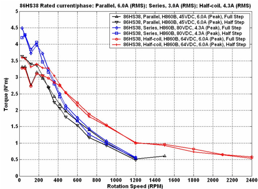
Figure 9: Speed-torque curves of the 86HS38
