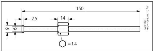
Figure 2: Weld nipple for KP-A
