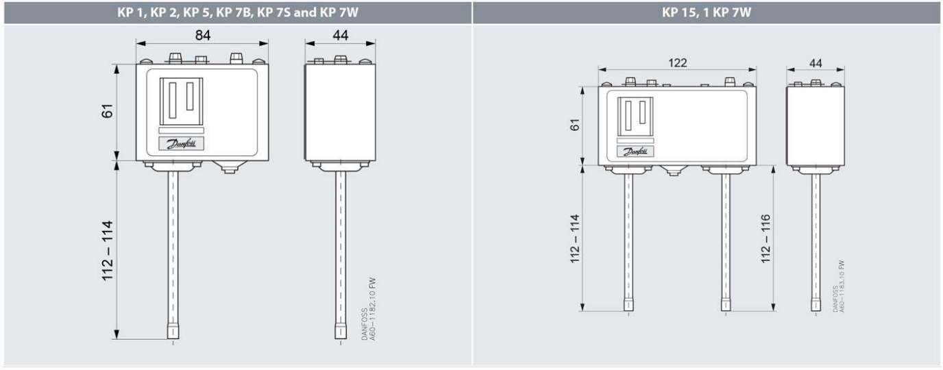
Figure 1: KP with top cover
