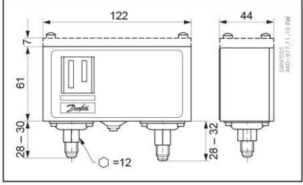
Figure 1: KP with top cover
