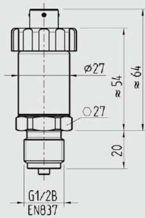
with bayonet connector (6-pin)
