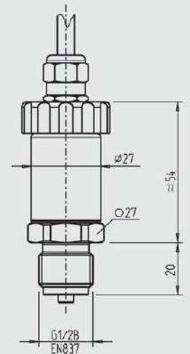
with cable outlet, standard
