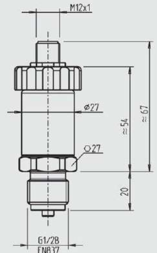
with circular connector M12 x 1 (4-pin)
