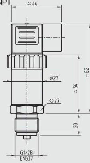
with angular connector DIN 175301-803 with 1/2 NPT
