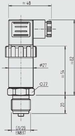
with angular connector DIN 175301-803 A
